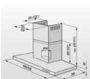
MORA 5705 (*60CM)
